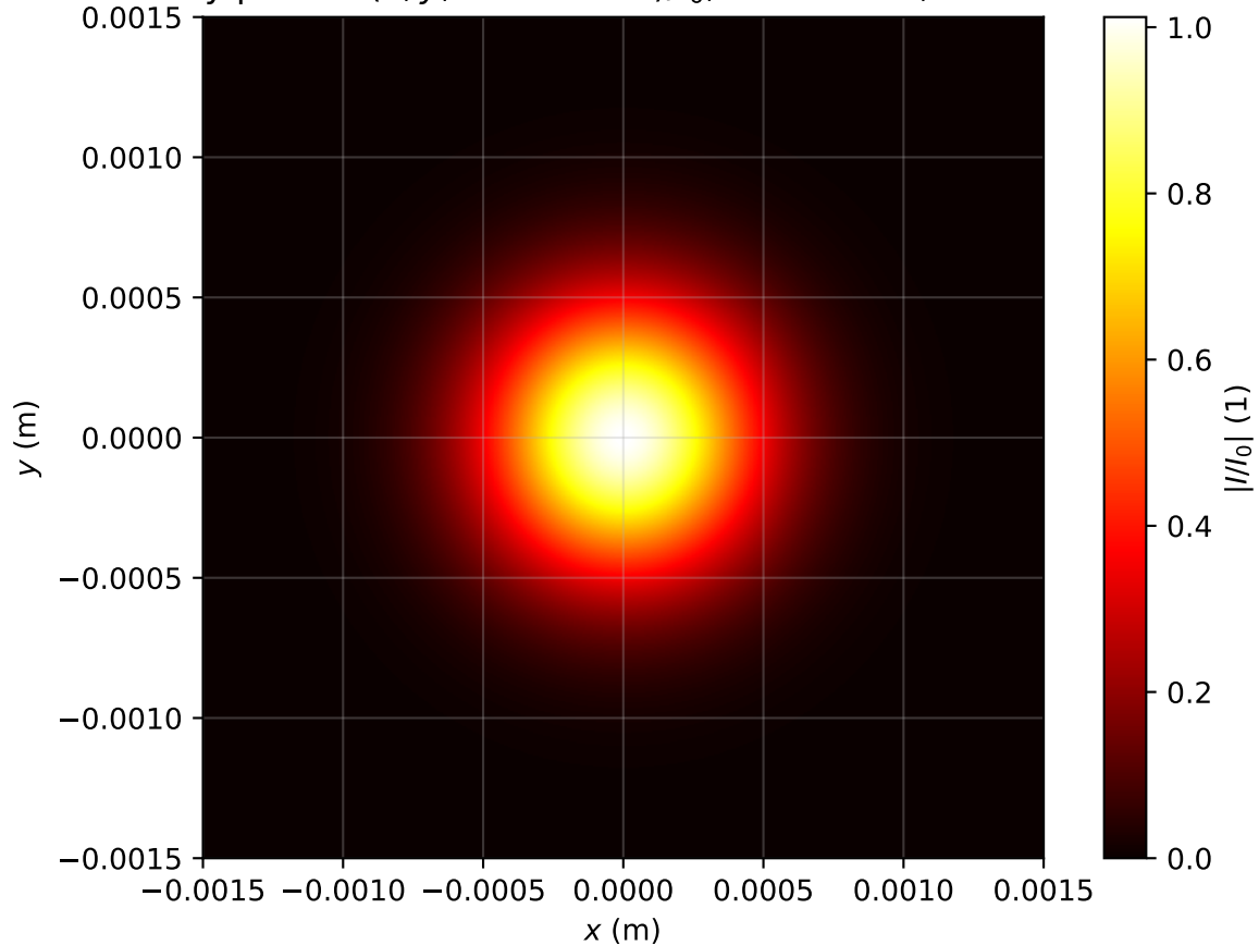
Intensity profile I(x, y, z = 0.318m)/I_0 , P_{in}=0.4P_{cr} , artificial time
